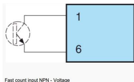
Fast count input NPN - Voltage
