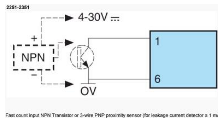
Fast count input NPN Transistor or 3-wire PNP proximity sensor (for leakage current detector \leq 1 mA)
