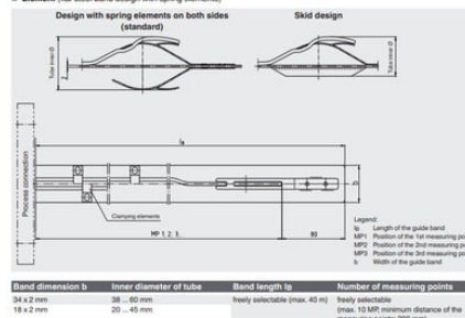
■ Element (flat-steel band design with spring elements)
