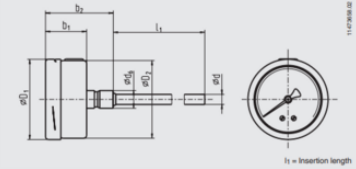
Model A70, back mount (NS 63)
