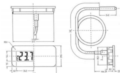
TF-LCD Solar
