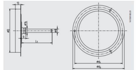
Smooth connection, with rear mounting flange
