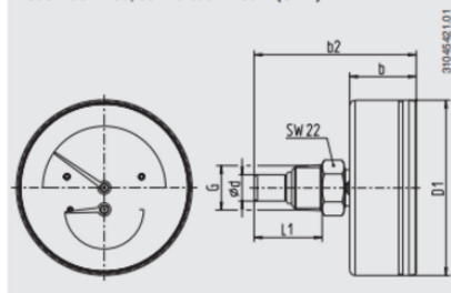
Model 100.12.80, centre back mount (CBM)
