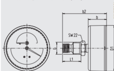
Model 100.02.80, centre back mount (CBM)
