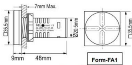
Outline Dimension
