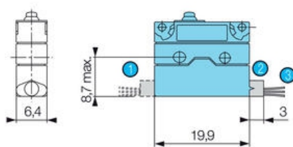
Cable Outputs
