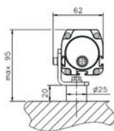
Angled fixing bracket + Antivibration support
