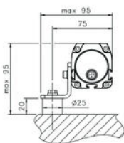
Angled fixing bracket + Antivibration support
