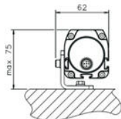
MOUNTING B
