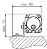
MOUNTING A
