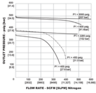
CP320 - Linear P1 pressures (CP3214022000-001)
