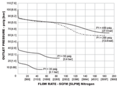
CP3200 - Lower PI pressures (CP3214022000-001)
