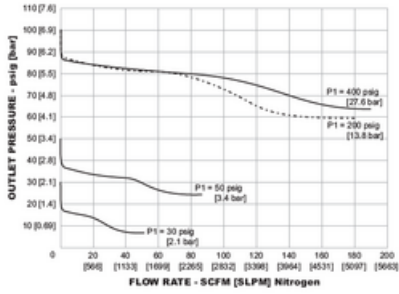
CP320 - Linear P1 pressures (CP3214022000-001)
