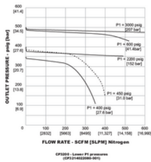
CP3200 - Lower PI pressures (CP3214022000-001)
