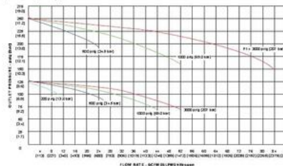
Cy = 0,06 Model Neoprene Diaphragm
