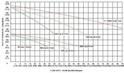
Cy = 0,20 Model Metal Diaphragm
