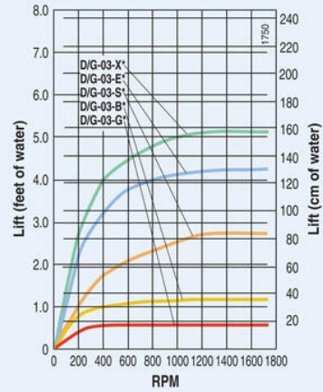
Dry Lift
