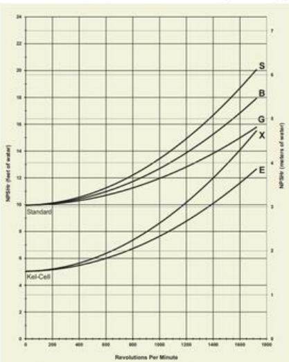
Net Positive Suction Head (NPSHr)
