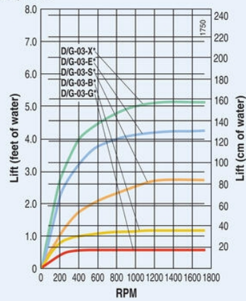
Dry Lift
