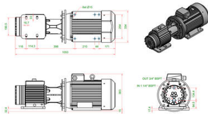
G15 Models with Metallic Pump Head mm (Inches)
