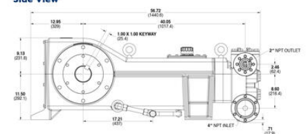
Threaded Version Inches (mm) Side View
