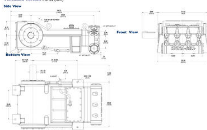
Threaded Version Inches (mm)
