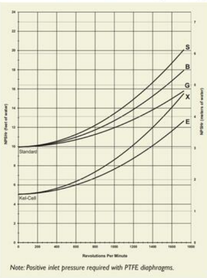
Net Positive Suction Head (NPSHr)
