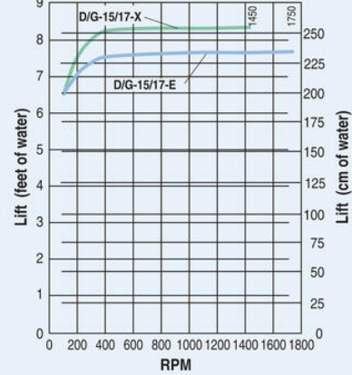
Dry Lift
