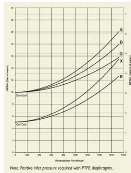
Net Positive Suction Head (NPSHr)
