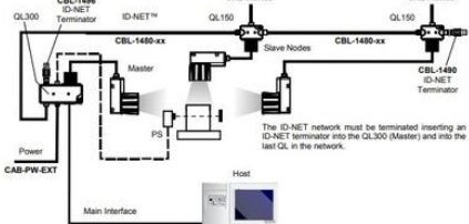
ID-NET™ Synchronized Network - Matrix 400™ Master with QL300 + Matrix 400™ Slaves with QL150
