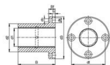
Dimensions [mm]
