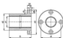
Dimensions [mm]
