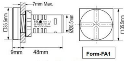
Outline Dimension
