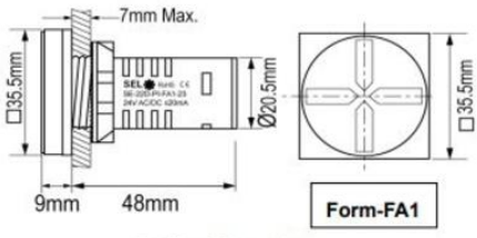
Outline Dimension
