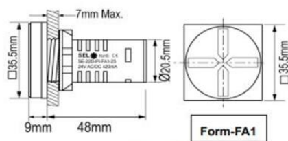
Outline Dimension
