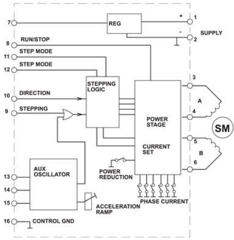
EM-186 BLOCK DIAGRAM
