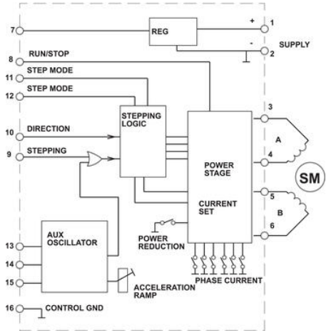
EM-186 BLOCK DIAGRAM
