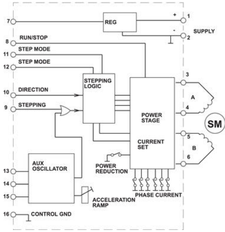
EM-186 BLOCK DIAGRAM
