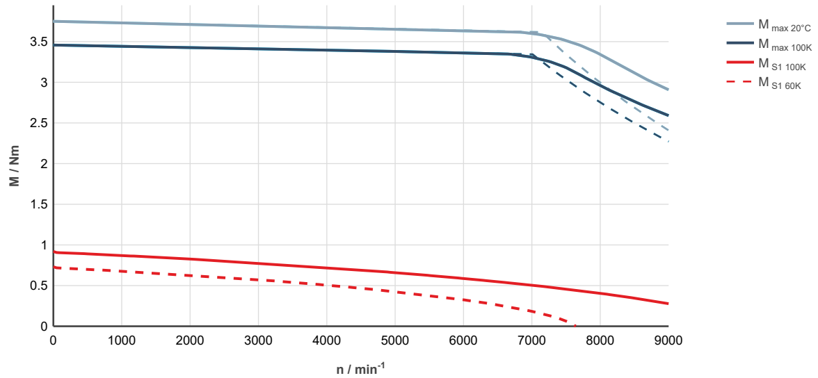
Fig. 17: MS2S03-B0BYN-___0-___-_, ctrlX DRIVE, controlled supply 3 x AC 400 ... 480 V
