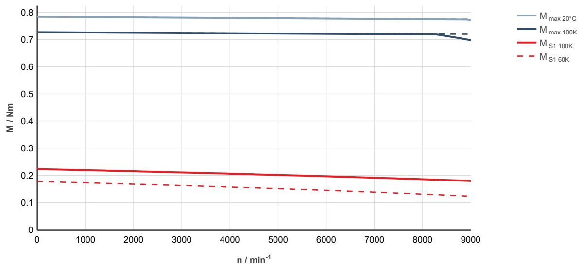
Fig. 12: MS2S02-A0BYN-___0-__N, ctrlX DRIVE, controlled supply 3 x AC 400... 480 V
