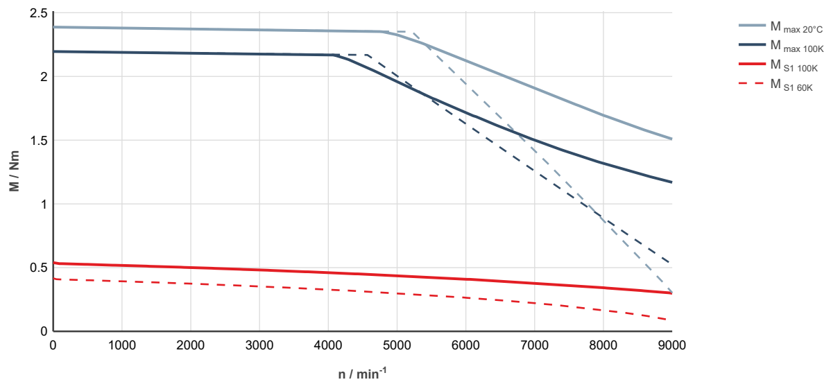
Fig. 13: MS2S02-C0BYN-___0-___-___, ctrlX DRIVE, uncontrolled supply 3 × AC 400 V
