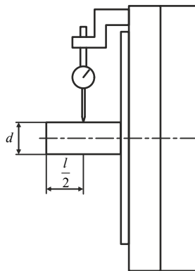
Fig. 3: Measuring system of concentricity tolerance
