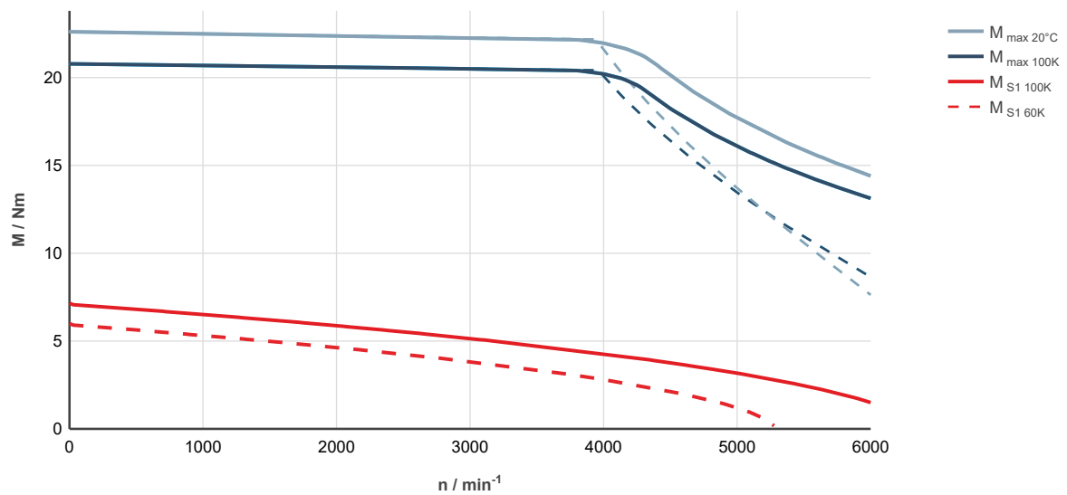
Fig. 28: MS2S05-C0BTN-___0-___-___, ctrlX DRIVE, uncontrolled supply 3 x AC 400 V
