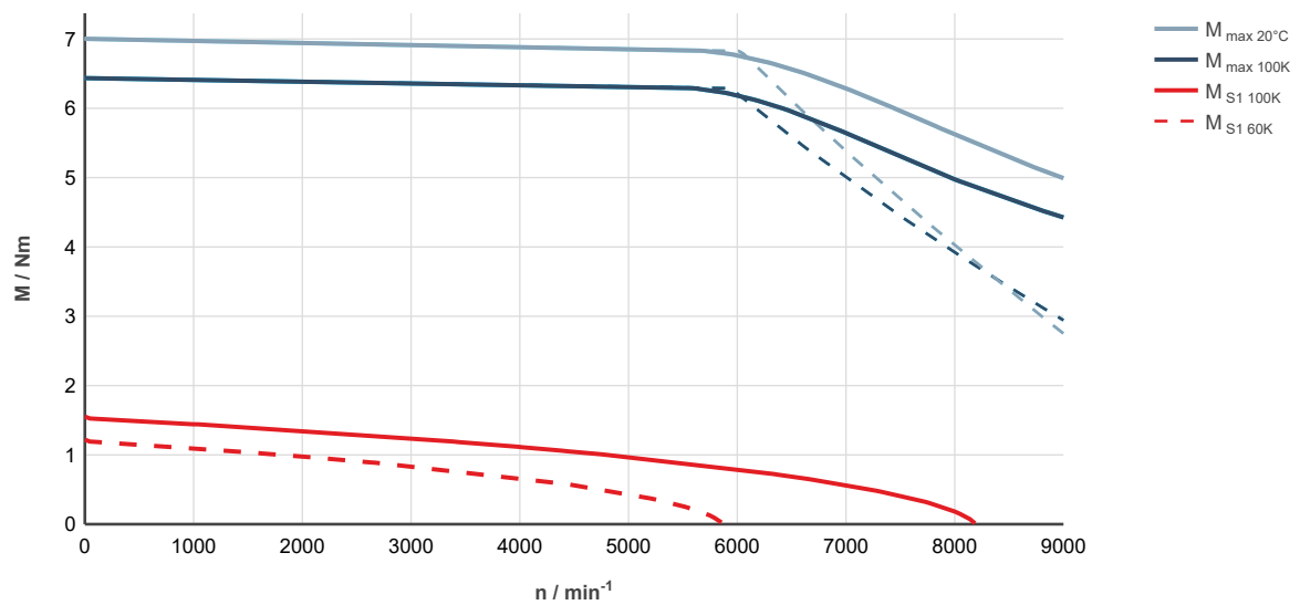
Fig. 18: MS2S03-C0BYN-___0-___-___, ctrlX DRIVE, uncontrolled supply 3 x AC 400 V
