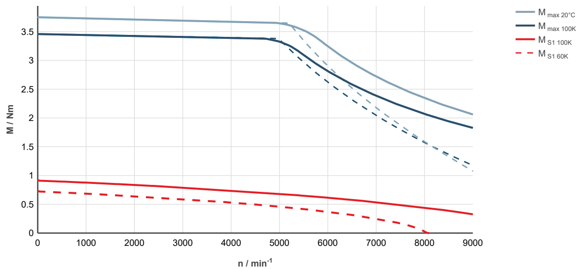
Fig. 16: MS2S03-B0BYN-___0-___-_, ctrlX DRIVE, uncontrolled supply 3 × AC 400 V
