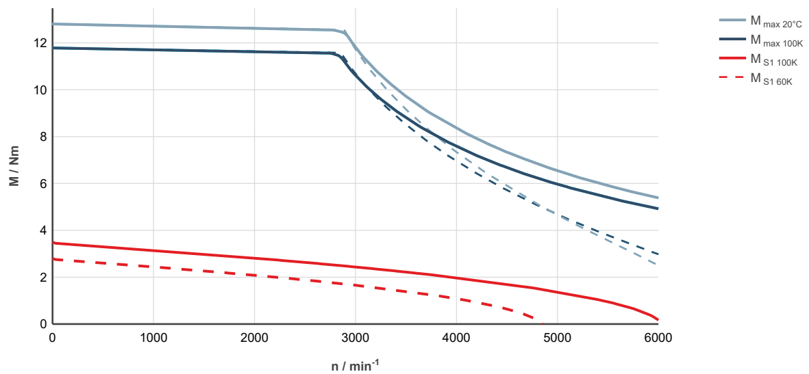
Fig. 23: MS2S04-C0BTN-___0-___-_, ctrlX DRIVE, uncontrolled supply 3 × AC 400 V
