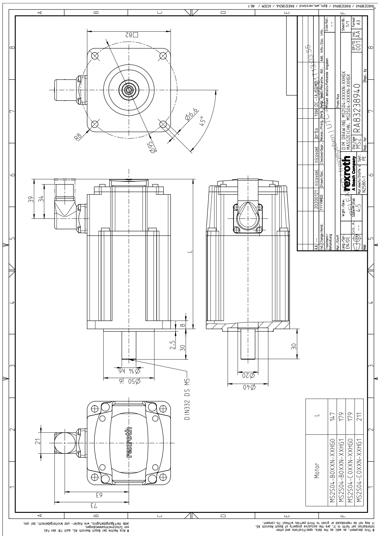
Fig. 25: MS2S04-XXXXN-XXHGX
