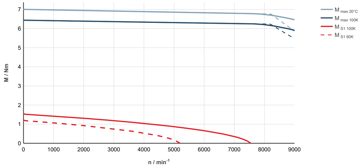
Fig. 19: MS2S03-C0BYN-___0-___-___, ctrlX DRIVE, controlled supply 3 x AC 400 ... 480 V
