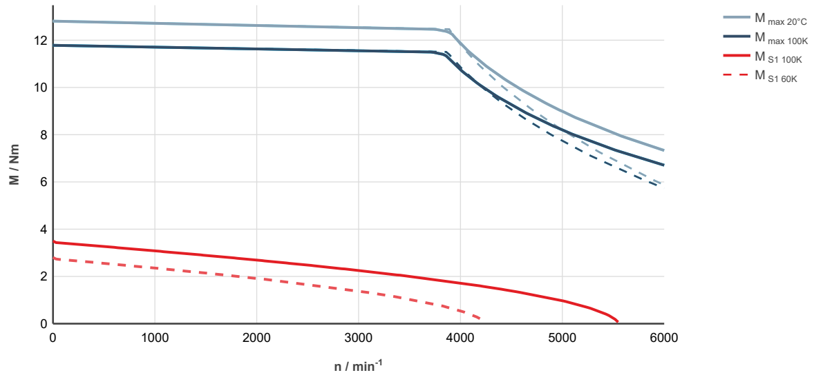
Fig. 24: MS2S04-C0BTN-___0-___-_, ctrlX DRIVE, controlled supply 3 x AC 400 ... 480 V
