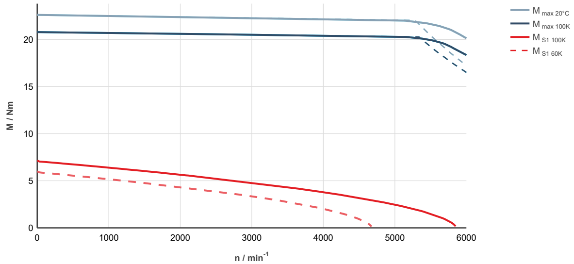
Fig. 29: MS2S05-C0BTN-___0-___-___, ctrlX DRIVE, controlled supply 3 x AC 400 ... 480 V
