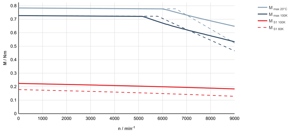
Fig. 11: MS2S02-A0BYN-___0-__N, ctrlX DRIVE, uncontrolled supply 3 × AC 400 V
