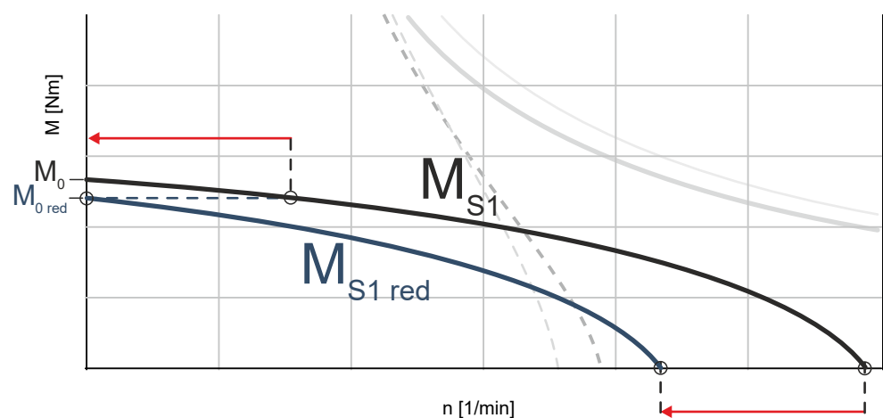
Fig. 34: Determine S1-characteristic curve M_{S1\ red} with derating factor f_{TH}
