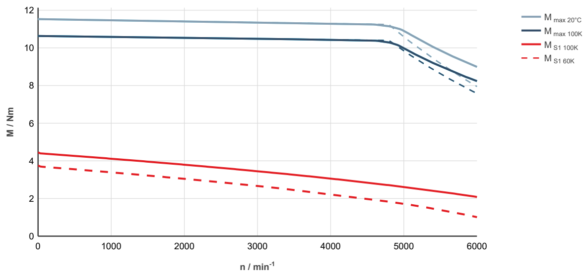
Fig. 27: MS2S05-B0BTN-___0-___-_, ctrlX DRIVE, controlled supply 3 x AC 400 ... 480 V
