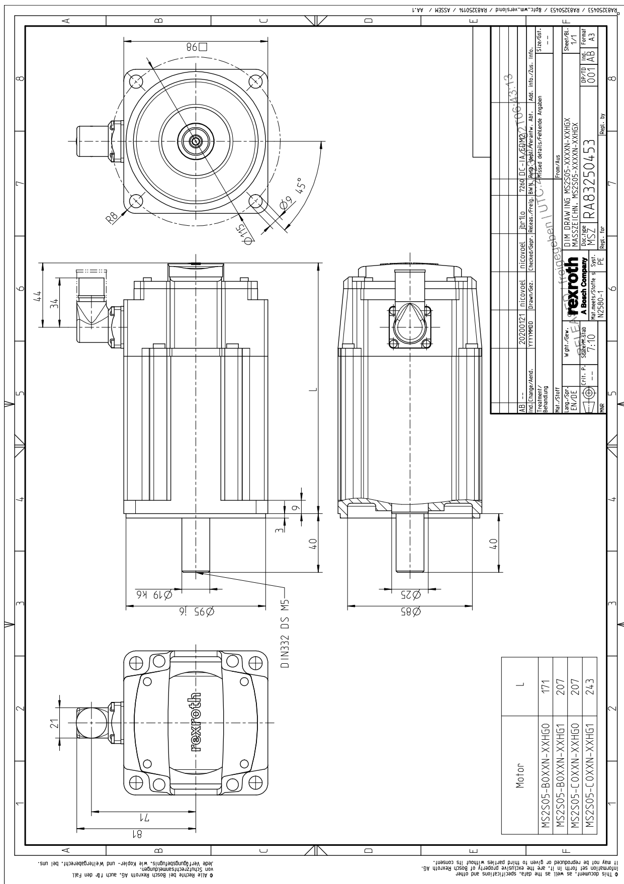
Fig. 30: MS2S05-XXXXN-XXHGX
