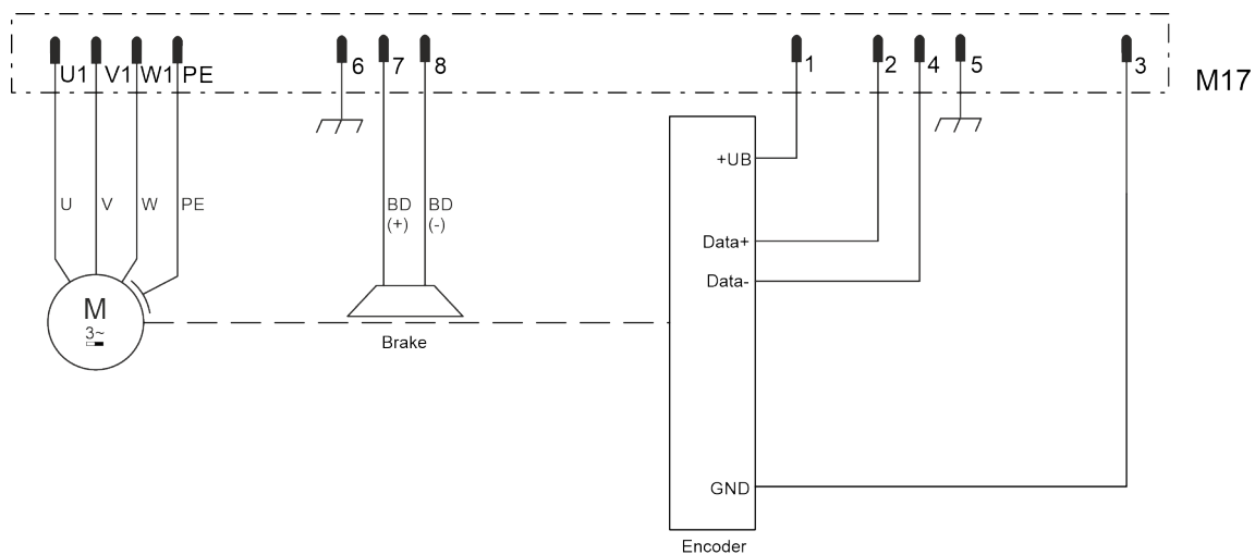
Fig. 31: Circuit diagram MS2S
