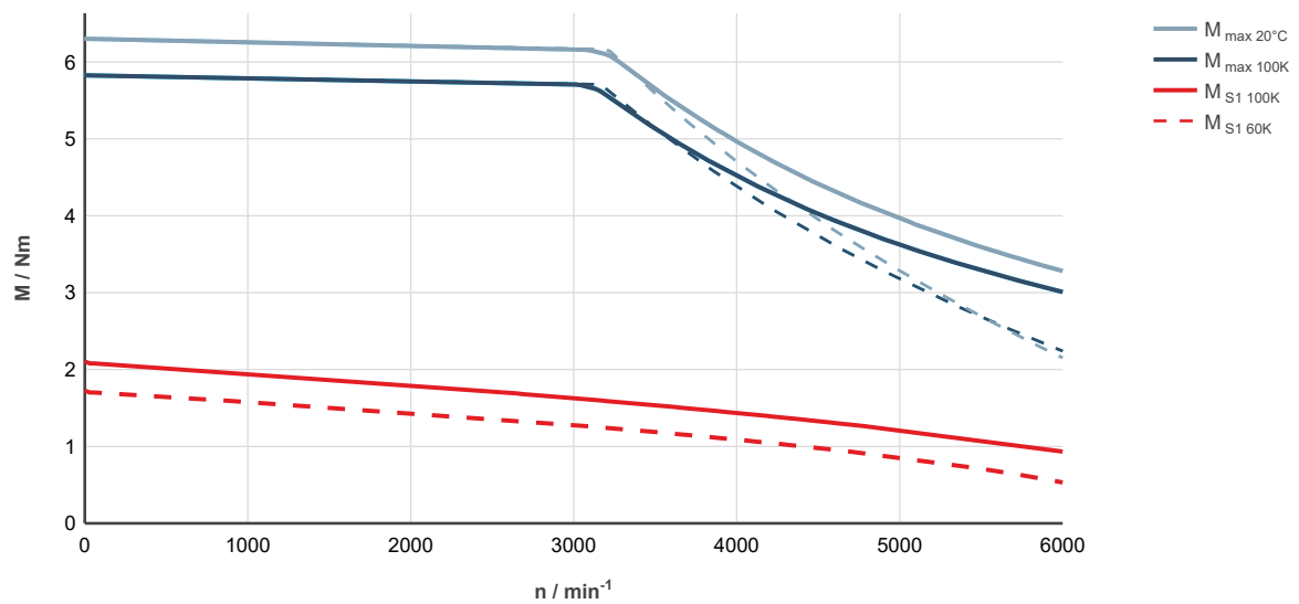
Fig. 21: MS2S04-B0BTN-___0-___-__, ctrlX DRIVE, uncontrolled supply 3 × AC 400 V
