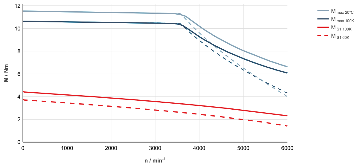
Fig. 26: MS2S05-B0BTN-___0-___-_, ctrlX DRIVE, uncontrolled supply 3 x AC 400 V
