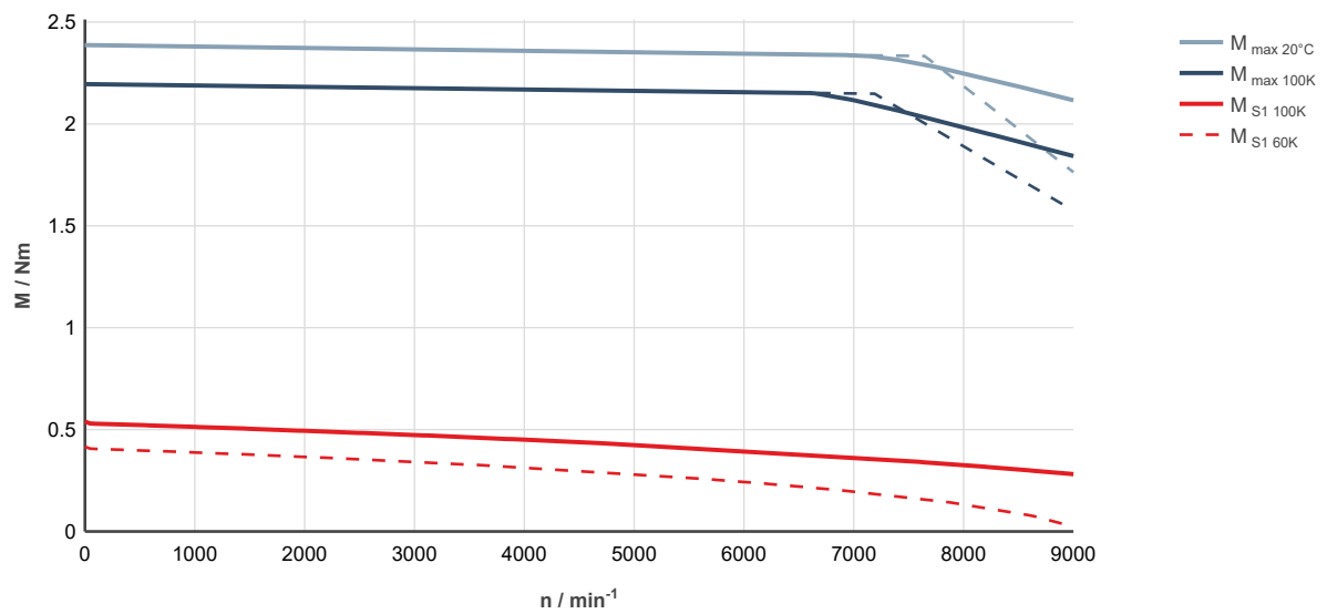
Fig. 14: MS2S02-C0BYN-___0-___-___, ctrlX DRIVE, controlled supply 3 x AC 400... 480 V
