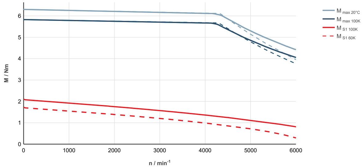
Fig. 22: MS2S04-B0BTN-___0-___-__, ctrlX DRIVE, controlled supply 3 x AC 400 ... 480 V
