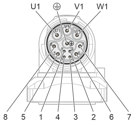
Fig. 32: Cable view of single cable connection M17
